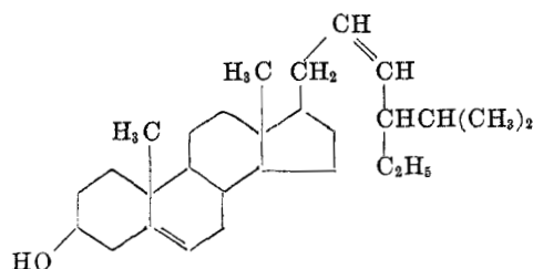
II Stigmasterol
